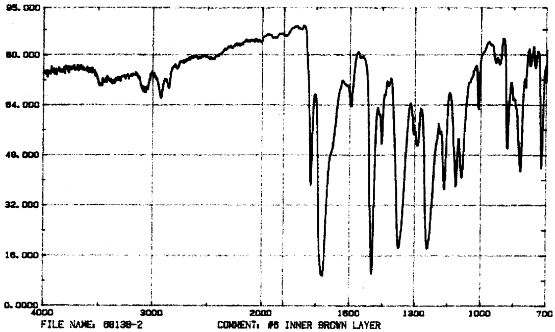
Figure 10. FTIR spectrum of the middle amber or brown insulation layer.
