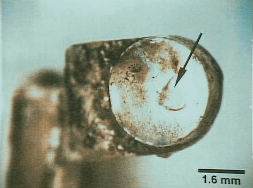
Systems 9 - Exhibit No. 9B - Photo 9. Figure 9c. The stationary line contact of the SPR circuit breaker has a tarnished appearance. Arrow highlights the mechanical wear from the making and breaking of the contacts.
