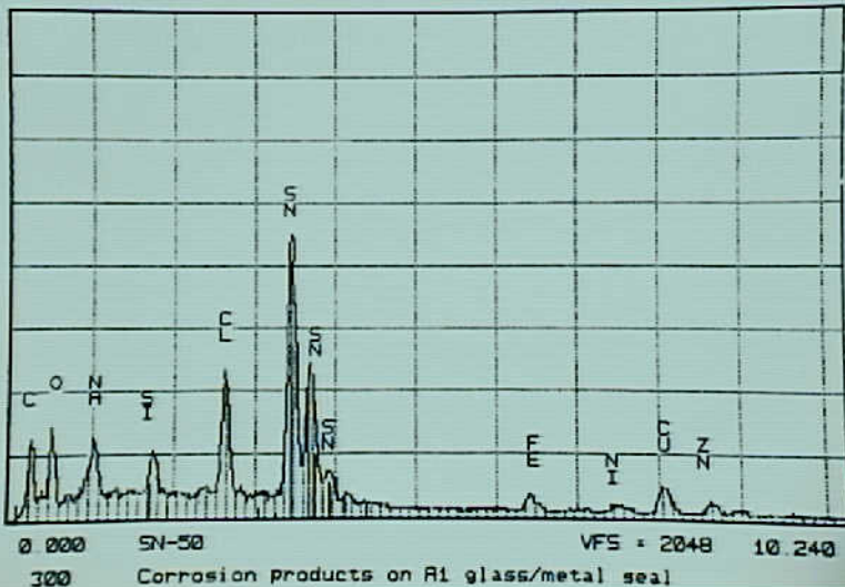
Systems 9 - Exhibit No. 9B - Photo 9. Figure 9b. Corrosion products on glass to metal seal of N.O.
