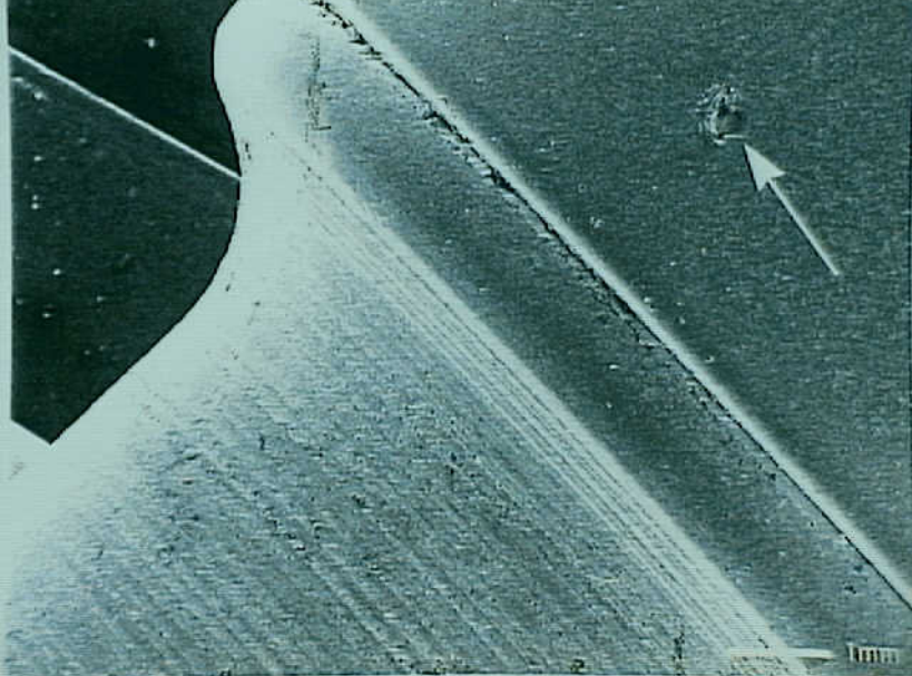
Systems 9 - Exhibit No. 9B - Photo 9. Figure 9a. SEM view of the gouge found on the scavenge pump switch knob (arrow).
