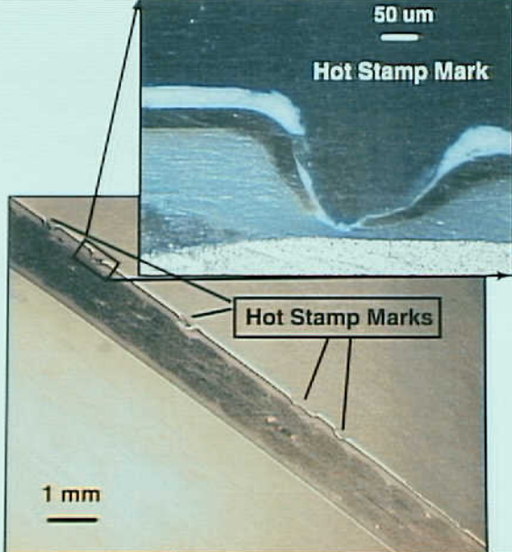
Systems 9 - Exhibit No. 9B - Photo 8. Figure 8f. Lateral cross section of a different wire than from figure 7. Again note depth variability of the mark from right to left. Note all three insulation layers were again penetrated.
