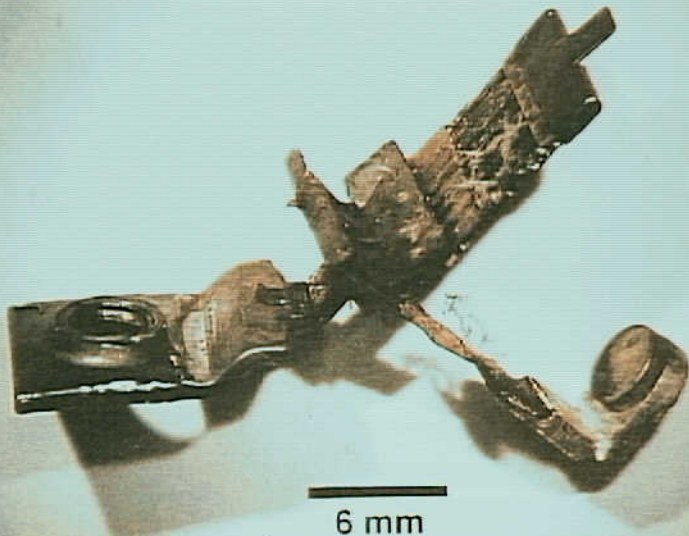
Systems 9 - Exhibit No. 9B - Photo 8. Figure 8c. The stationary load terminal and contact of the SPR circuit breaker have a tarnished appearance.
