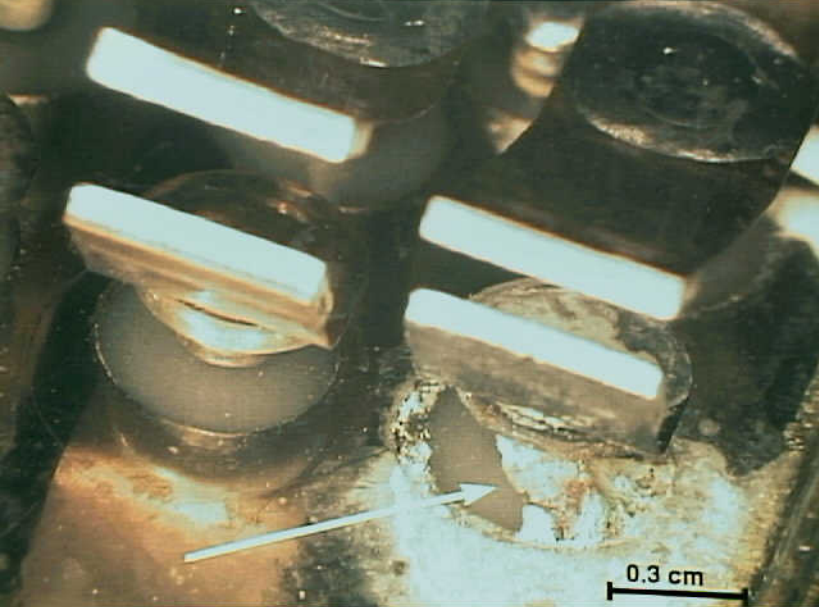
Systems 9 - Exhibit No. 9B - Photo 8. Figure 8b. Residues on and surrounding the glass to metal seal of N.O. contact A1.
