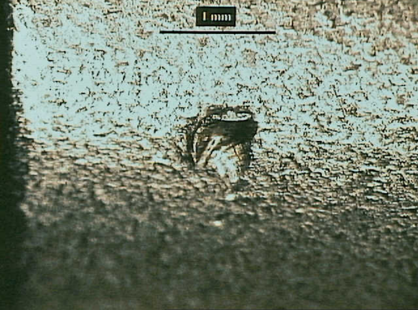
Systems 9 - Exhibit No. 9B - Photo 8. Figure 8a. Close-up of the gouge. Note the metal displacement used to determine the gouge direction.
