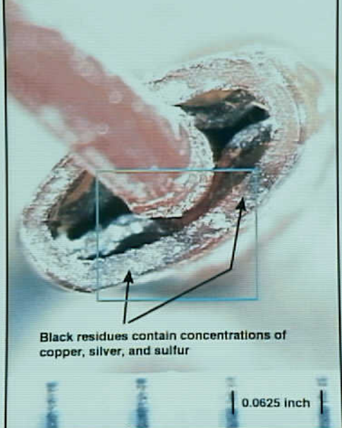
Systems 9 - Exhibit No. 9B - Photo 7. Figure 7g. Lo-Z lead wire crimp-on ring connector from N93119, sample #22.
