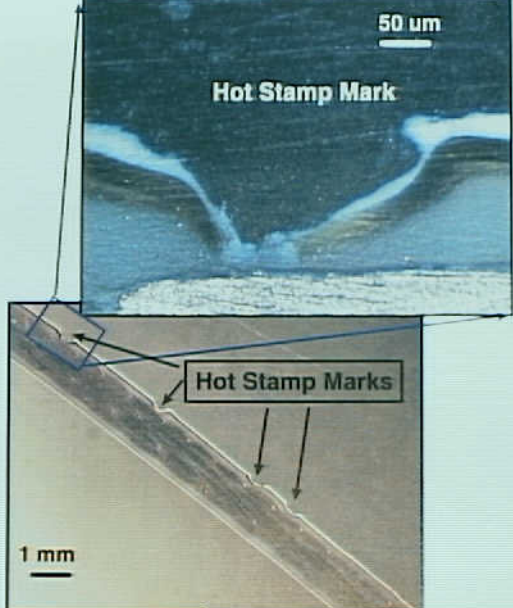
Systems 9 - Exhibit No. 9B - Photo 7. Figure 7f. Lateral cross section showing multiple hot stamp sites. Note variability of depth penetration from right to left. Note close-up of upper left mark showing the mark penetrated all three insulation layers.
