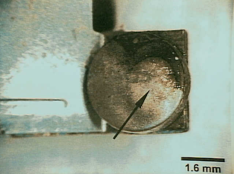
Systems 9 - Exhibit No. 9B - Photo 6. Figure 6c. The moving load contact of the SPR circuit breaker has a tarnished appearance. The arrow highlights the mechanical wear from making and breaking of the
