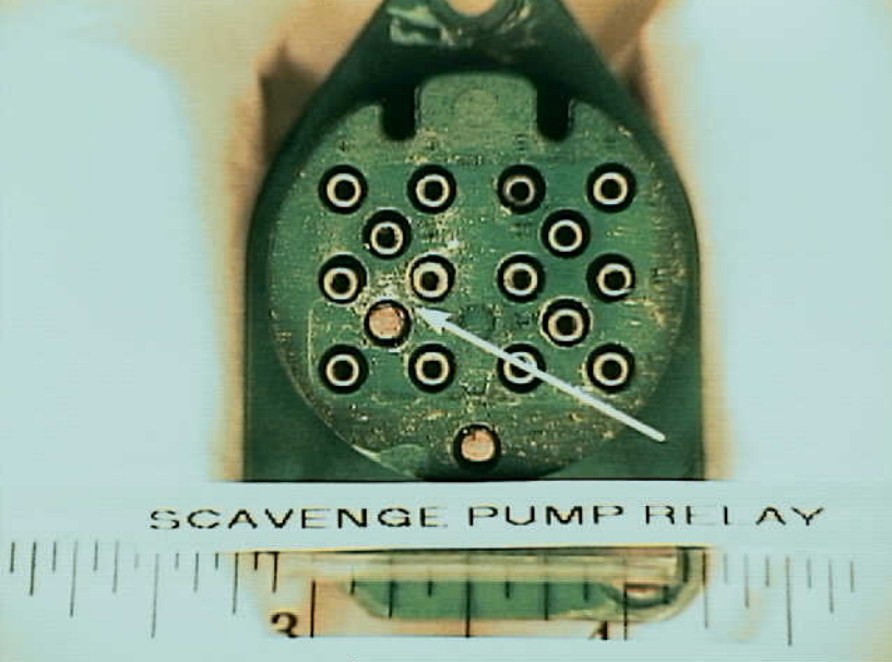
Systems 9 - Exhibit No. 9B - Photo 6. Figure 6b. Electrical connector. Arrow shows the white residue on the mating surface.
