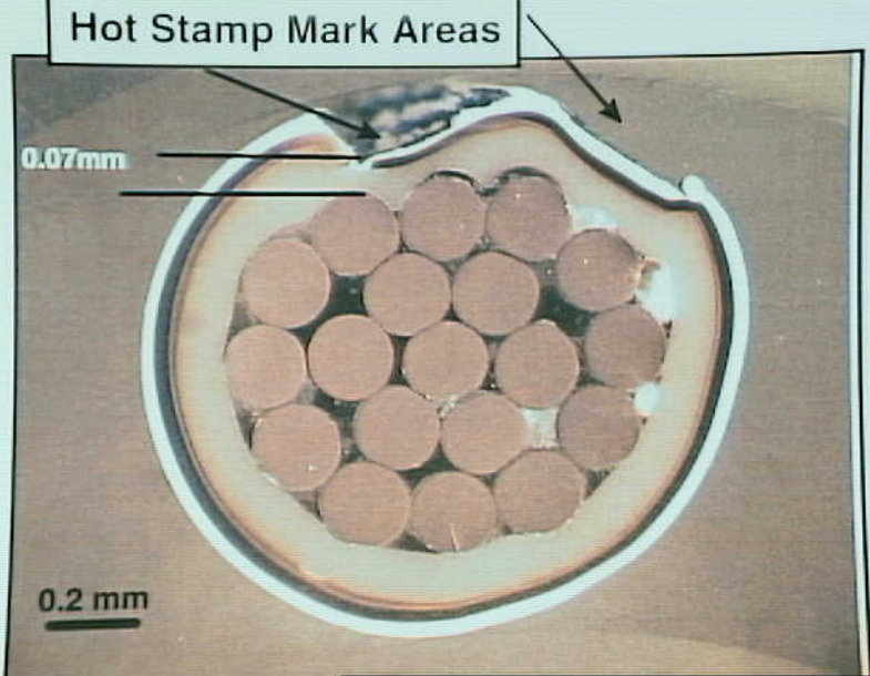
Systems 9 - Exhibit No. 9B - Photo 6. Figure 6f. Perpendicular cross section showing depth penetration of the hot stamp marks. Note that all three insulation layers were penetrated and the inner white layer was deformed by the stamping process.
