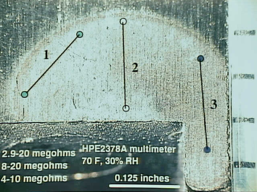
Systems 9 - Exhibit No. 9B - Photo 54. Figure 54g. Lower edge of Hi-Z terminal block from fuel probe FG420A12 A-14 (white arrow, Figure 52). Resistance of the residue was in the the megohm range using a multimeter (1.5Vdc).
