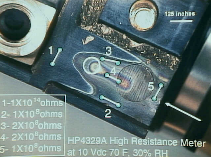
Systems 9 - Exhibit No. 9B - Photo 52. Figure 52g. Hi-Z location on terminal block from probe FG420A12, A-14. Note residue on surface and low electrical resistance. Residue contained high concentrations of silver, copper, and sulfur.
