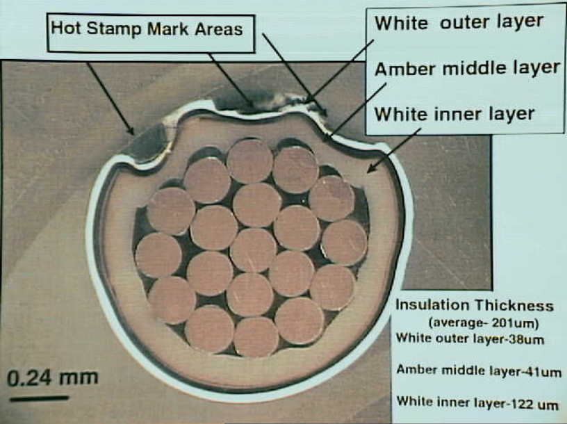
Systems 9 - Exhibit No. 9B - Photo 5. Figure 5f. Cross section of the wire showing three layer construction and depth penetration of the hot stamp mark. Note thickness of layers and total thickness at bottom right. Note deformation in inner layer.
