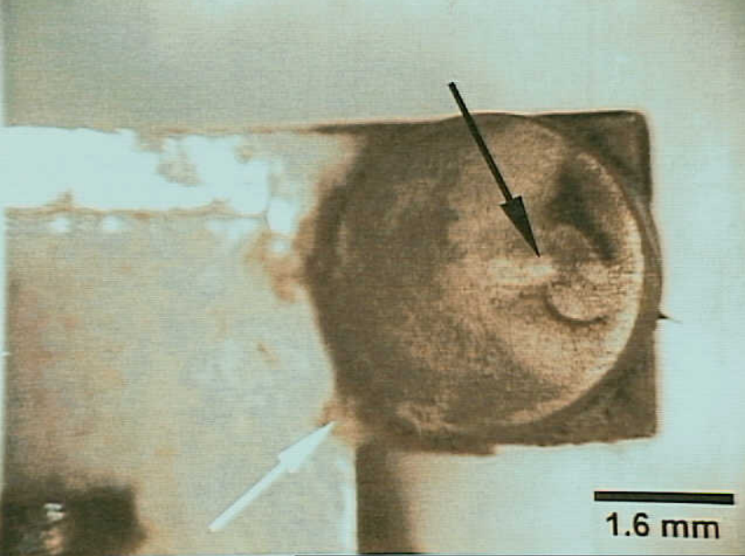
Systems 9 - Exhibit No. 9B - Photo 5. Figure 5c. The moving line contact of the SPR circuit breaker has a tarnished appearance. Black arrow highlights mechanical wear from the making and breaking of the contacts. White arrow indicates the fibrous residue
