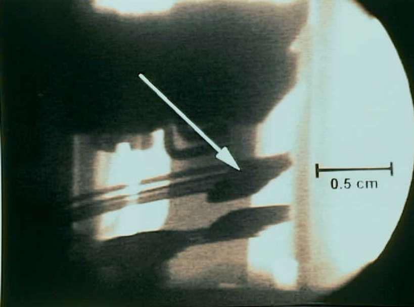
Systems 9 - Exhibit No. 9B - Photo 5. Figure 5b. Radiograph of relay. Arrow showing the N.O. contacts are open.
