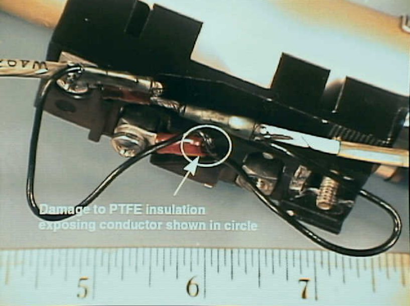
Systems 9 - Exhibit No. 9B - Photo 48. Figure 48g. Fuel probe (model no. FG420A12, serial no. A-9) from N93105 having apparent compression damage to PTFE insulation.
