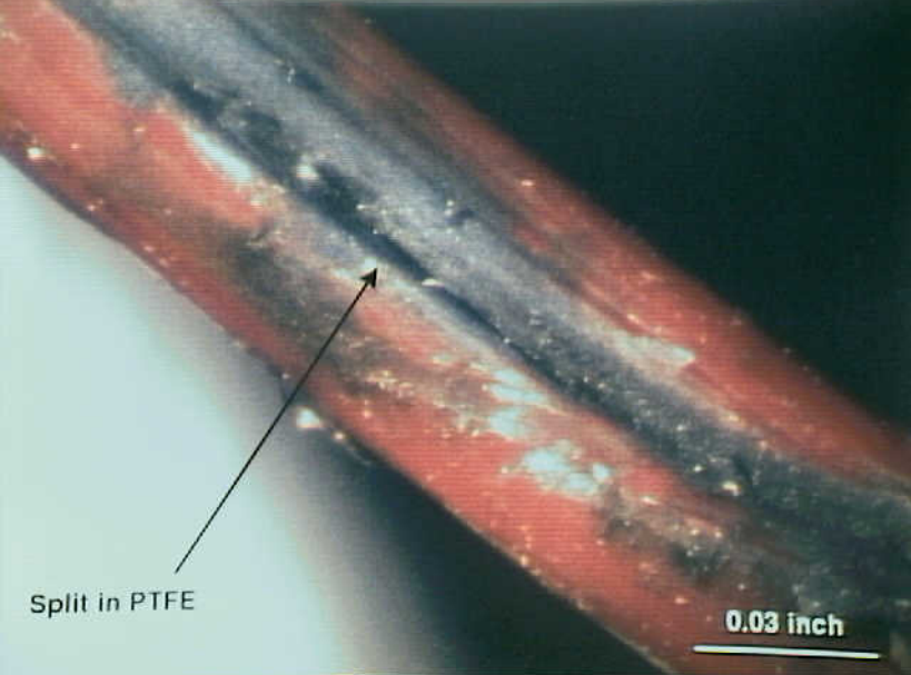
Systems 9 - Exhibit No. 9B - Photo 42. Figure 42g. Lo-Z wire from N93105 (model no. FG420A12, serial no. A-21).
