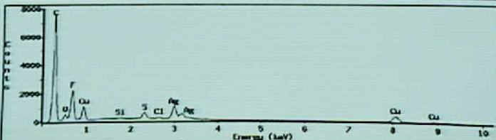
Systems 9 - Exhibit No. 9B - Photo 41. Figure 41g-2. Elemental X-ray microanalysis of film residue. Note high concentrations of copper, silver, and sulfur at points 1 and 2. These were taken on the film material. Point 3 was taken on the PTFE insulation.
