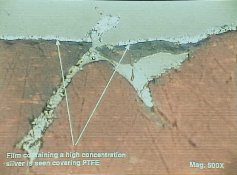
Systems 9 - Exhibit No. 9B - Photo 40. Figure 40g. Lo-Z wire from N93105 (model no. FG420A13, serial no. A-16) seen in Figures 38 and 39.
