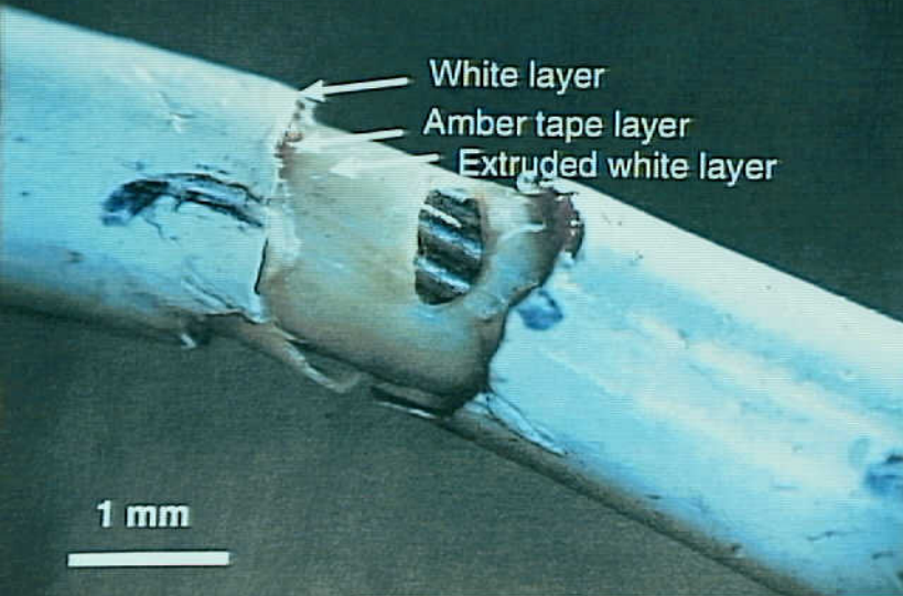
Systems 9 - Exhibit No. 9B - Photo 4. Figure 4d. Typical mechanically damaged insulation area. Note the damage reveals the multiple layered insulation
