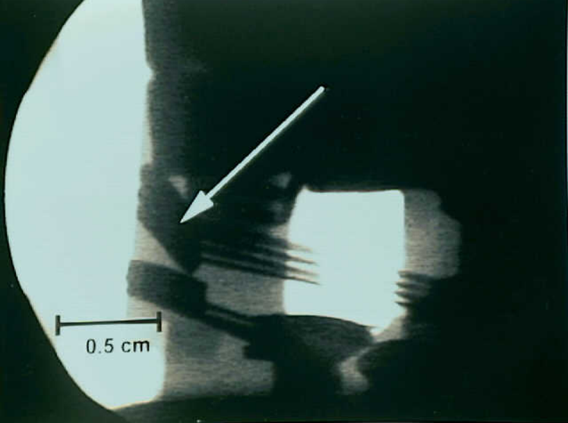
Systems 9 - Exhibit No. 9B - Photo 4. Figure 4b. Radiograph of relay. Arrow showing the N.C. contacts are open.
