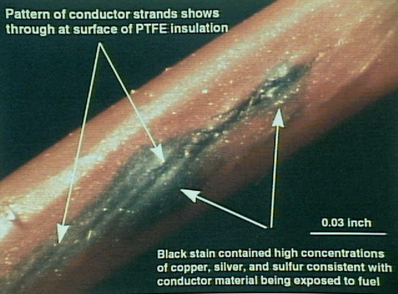
Systems 9 - Exhibit No. 9B - Photo 38. Figure 38g. Lo-Z wire from N93105 fuel probe (model no. FG420A13, serial no. A-16).
