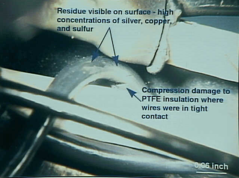
Systems 9 - Exhibit No. 9B - Photo 36. Figure 36g. Compensator (model no. FG6C1, serial no. 1-166) from N93105 having apparent compression damage to PTFE insulation.
