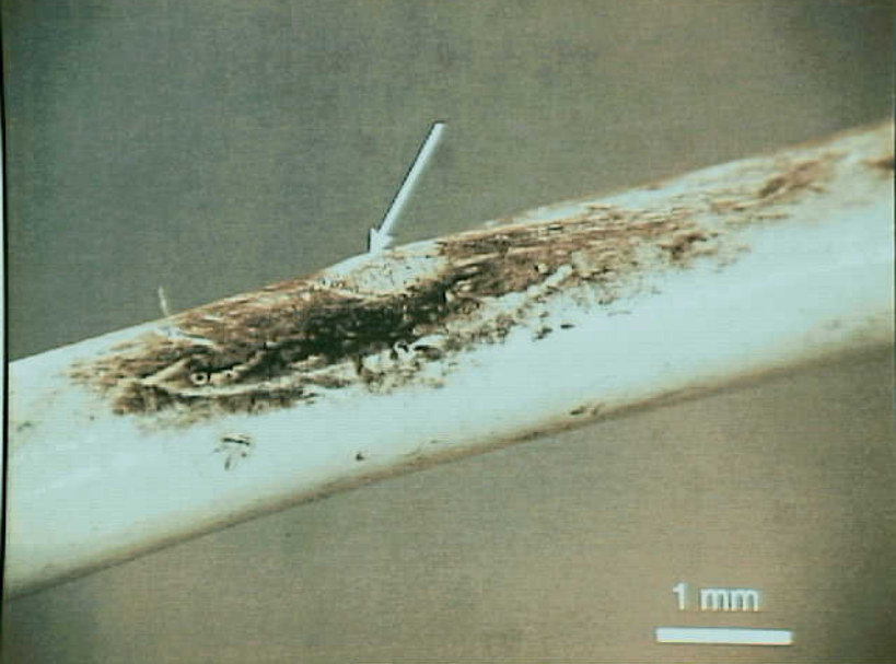
Systems 9 - Exhibit No. 9B - Photo 3. Figure 3d. Blackened and thermally damaged area on wiring. Note raised area (arrow).
