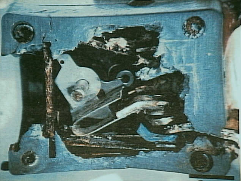
Systems 9 - Exhibit No. 9B - Photo 3. Figure 3c. Various mechanical components of the SPR circuit breakers are corroded. The moving contacts are lying against the stationary contacts.
