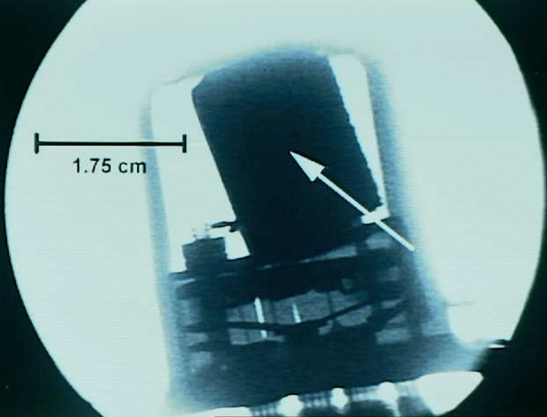
Systems 9 - Exhibit No. 9B - Photo 3. Figure 3b. Radiograph of relay. Arrow indicates the coil that is tilted off its axis.
