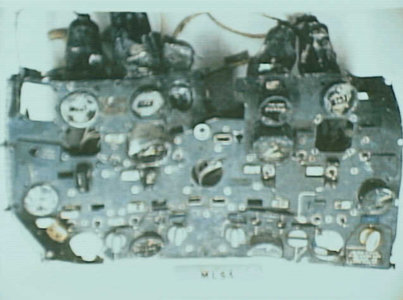
Systems 9 - Exhibit No. 9B - Photo 3. Figure 3a. Face side of flight engineer's fuel control panel as received.
