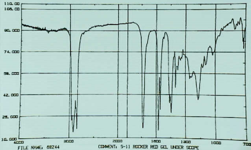
Systems 9 - Exhibit No. 9B - Photo 28. Graph 28. FTIR spectrum of the red lubricant in S-11 switch which was similar to the reference spectrum of ester-based lithium stearate.
