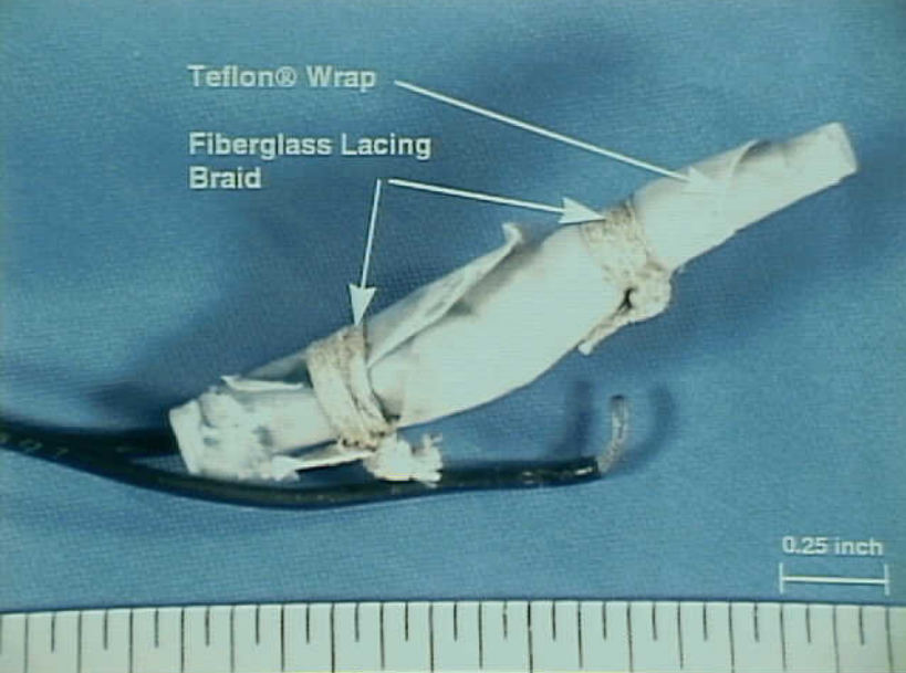
Systems 9 - Exhibit No. 9B - Photo 27. Figure 27g. Hi-Z pigtail lead from probe #31 out of N93119.
