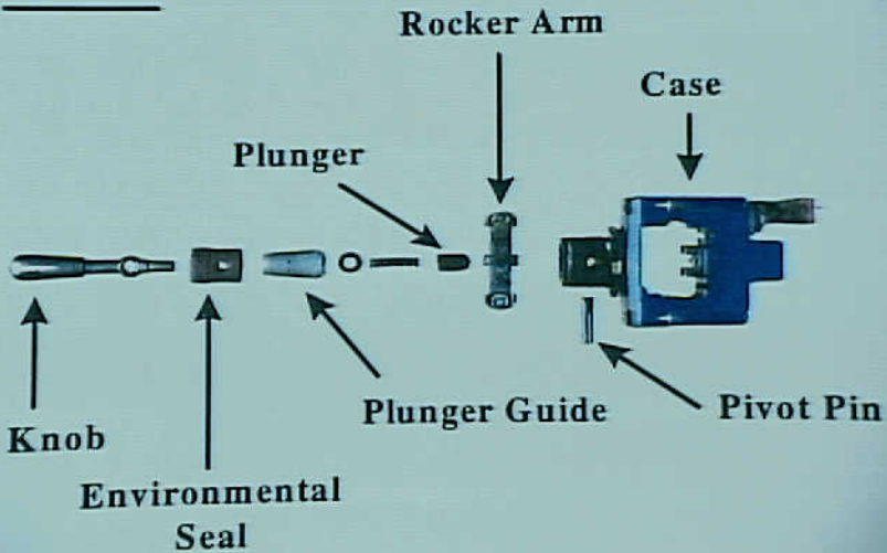
Systems 9 - Exhibit No. 9B - Photo 27. Figure 27a. Exploded view of switch S-11 following disassembly.
