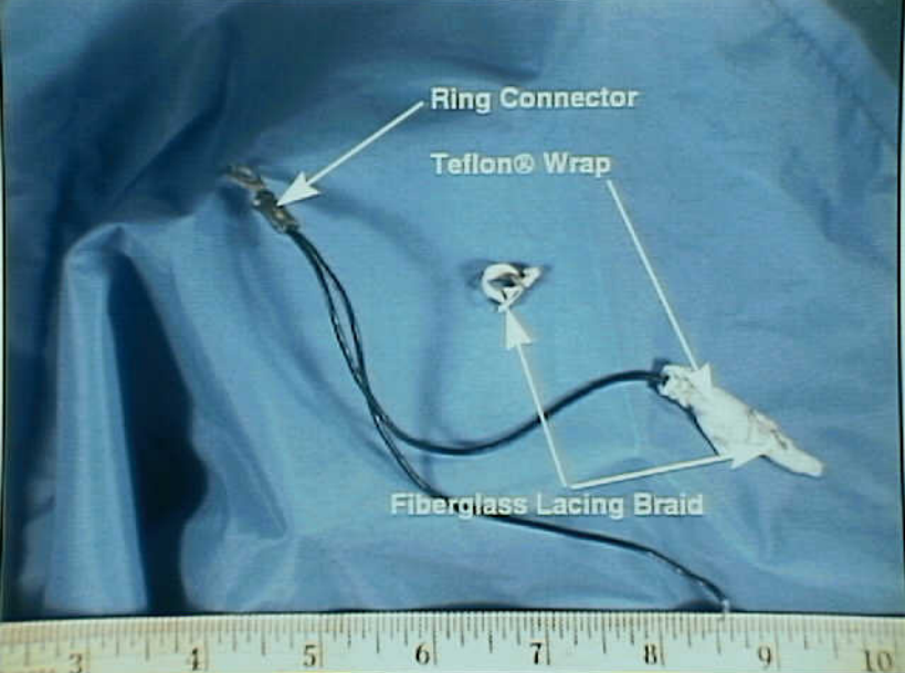
Systems 9 - Exhibit No. 9B - Photo 26. Figure 26g. Hi-Z pigtail leads from probe #31 out of N93119.
