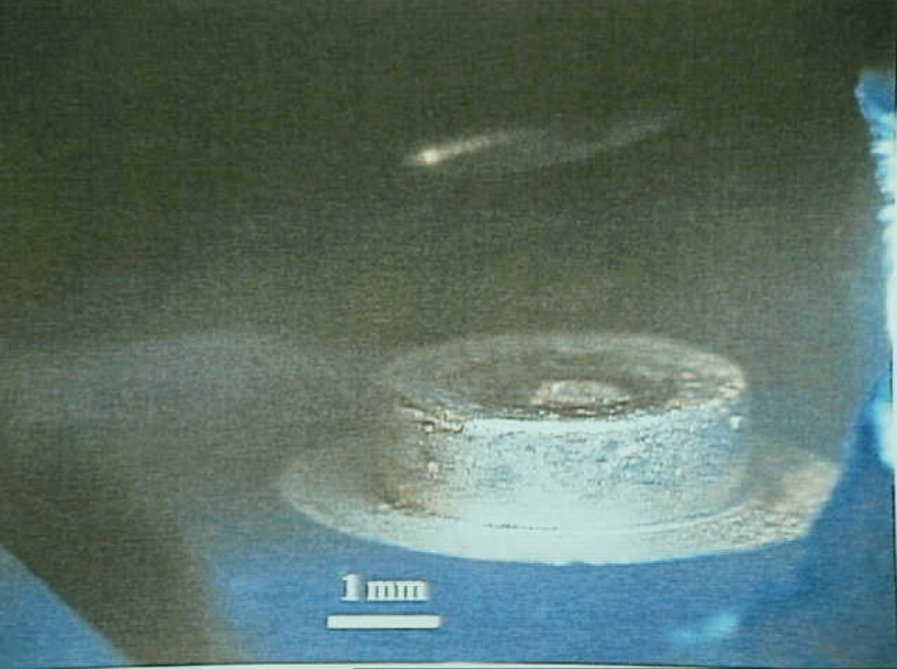
Systems 9 - Exhibit No. 9B - Photo 25. Figure 25a. Noormally closed stationary contact surface of the right jettison switch which exhibited little or no salt water-like residues.
