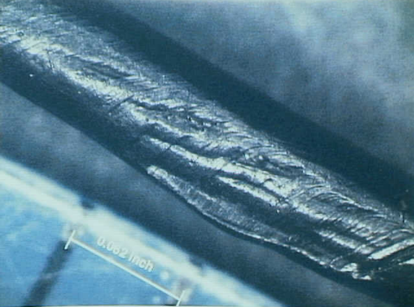
Systems 9 - Exhibit No. 9B - Photo 23. Figure 23g. Compression damage from strain relief clamp (N93110 compensator sample #45).
