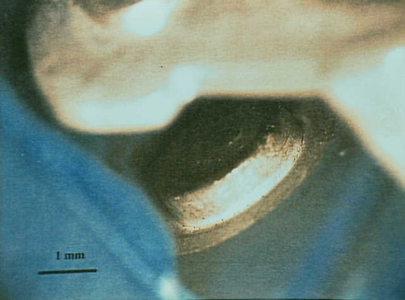
Systems 9 - Exhibit No. 9B - Photo 23. Figure 23a. Normally open contact surface from the left jettison switch exhibiting typical wear.
