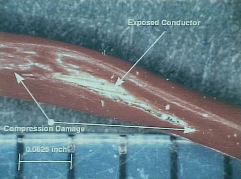
Systems 9 - Exhibit No. 9B - Photo 22. Figure 22g. Compression damage (N93119 sample #17).
