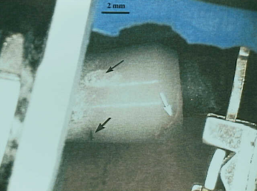
Systems 9 - Exhibit No. 9B - Photo 22. Figure 22a. Internal view of the plunger and guide, red lubricant, (at white arrow, chemically analyzed) and rocker arm of switch S11. Mold runner mark is apparent at the black
