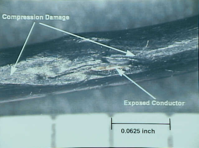
Systems 9 - Exhibit No. 9B - Photo 21. Figure 21g. Representative damage to a fuel probe wiring from
