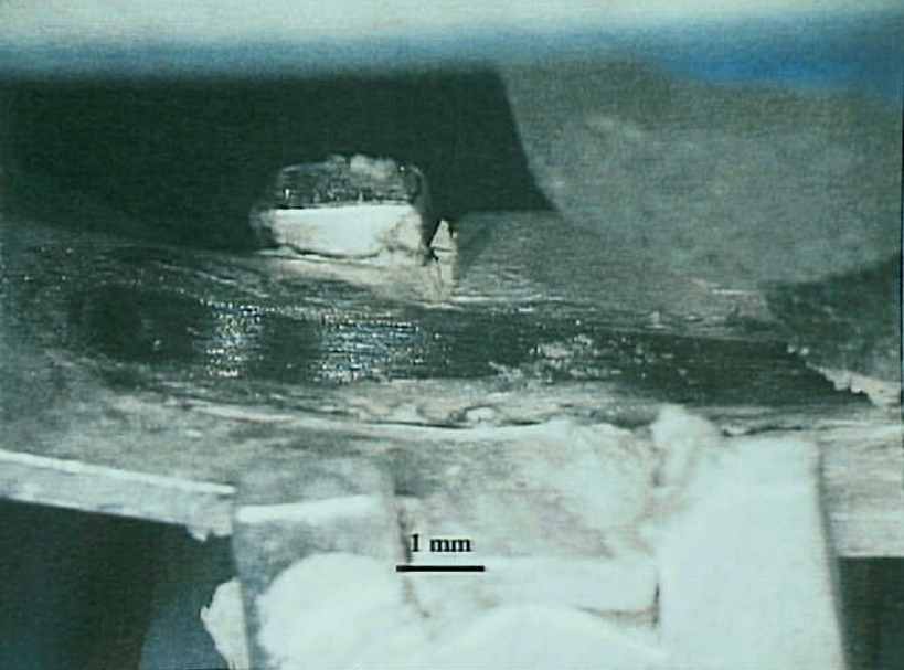
Systems 9 - Exhibit No. 9B - Photo 21. Figure 21a. Internal view of the switch mechanism of the right jettison switch.
