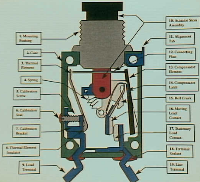
Systems 9 - Exhibit No. 9B - Photo 21. Appendix 1c. Circuit Breaker Parts Descriptions
