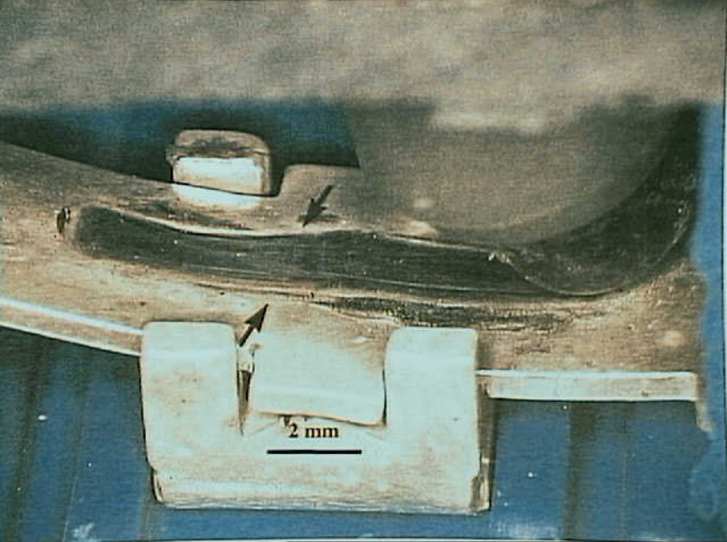
Systems 9 - Exhibit No. 9B - Photo 20. Figure 20a. Internal view of the switch mechanism of the left jettison switch. The track is apparent as indicated between the arrows.
