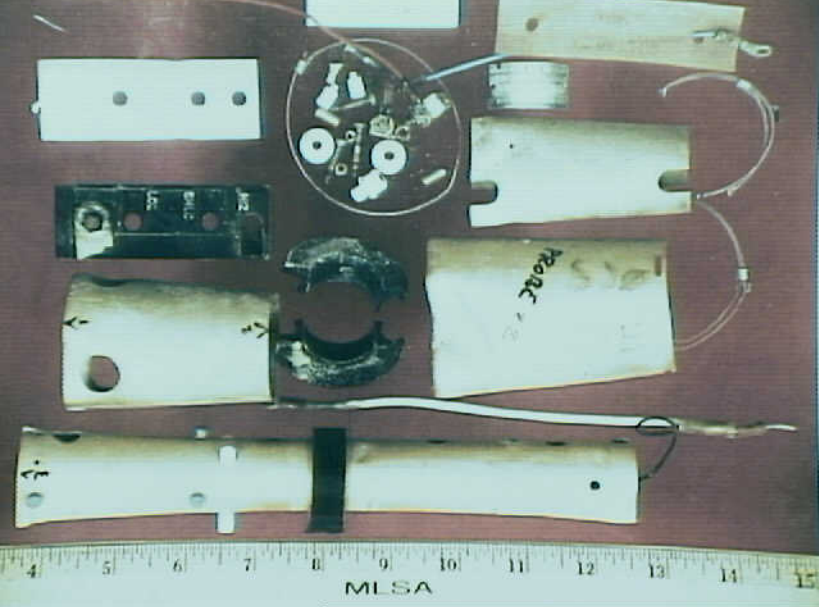
Systems 9 - Exhibit No. 9B - Photo 2. Figure 2g. Sample 22 from N93119 center tank. Typical damage to recovered fuel probe.
