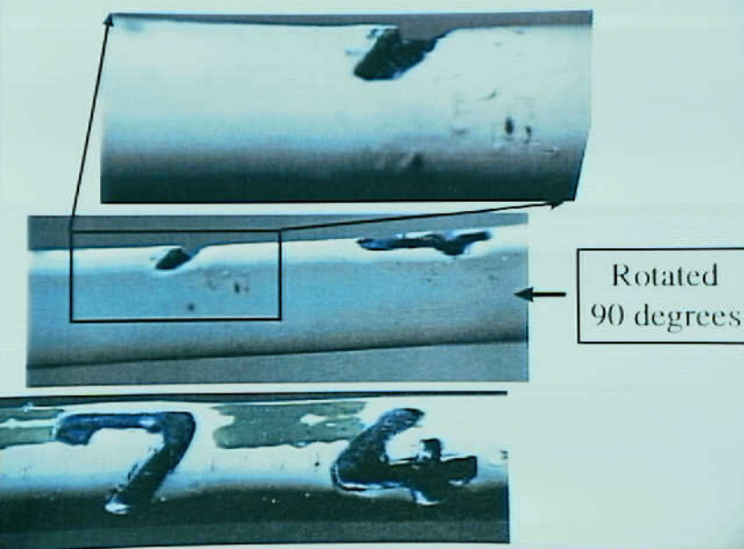
Systems 9 - Exhibit No. 9B - Photo 2. Figure 2f. Typical example of hot stamp markings on relay connector wiring. Note depth penetration of the mark. A close-up of the seven mark is shown at the top. Mag
