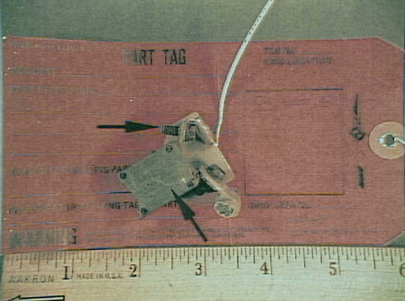
Systems 9 - Exhibit No. 9B - Photo 2. Figure 2c. As received condition of the SPR circuit breaker. The upper arrow highlights the corroded terminal hardware. The lower arrow highlights the cracked housing.
