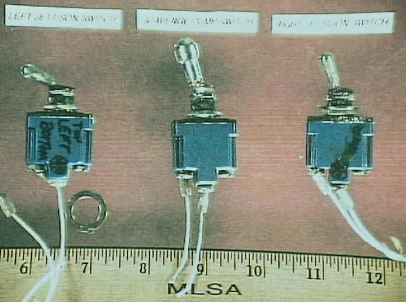
Systems 9 - Exhibit No. 9B - Photo 2. Figure 2a. Side 2 of the three switches received for analysis.
