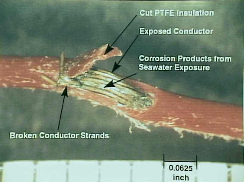
Systems 9 - Exhibit No. 9B - Photo 19. Figure 19g. Representative damage to a fuel probe wiring from
