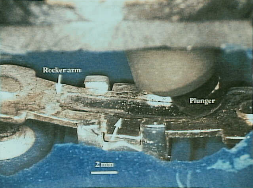
Systems 9 - Exhibit No. 9B - Photo 19. Figure 19a. Internal view of the scavenge pump switch mechanism. The arrow indicates the lubricant material on the rocker arm which was chemically analyzed.
