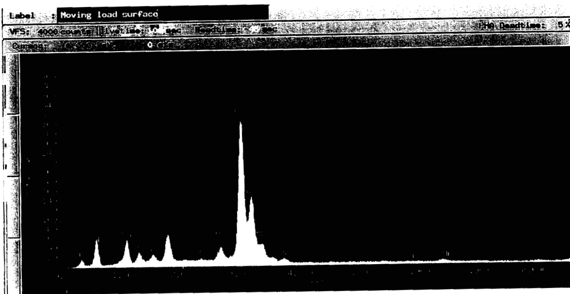
Figure 19. EDS spectrum of the moving load contact surface of the RTV circuit breaker. The silver in both spectrums is primarily from the contact material.
